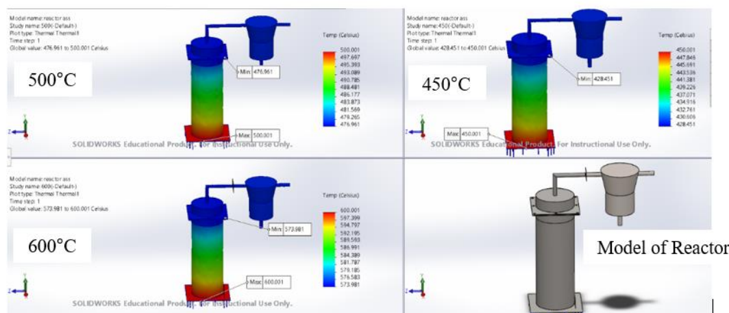
Figure 3. shows the model and simulation of the fixed bed reactors at three different temperatures of 450°C, 500°C and 600°C.
