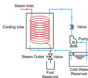
Figure 4. Condenser system design
