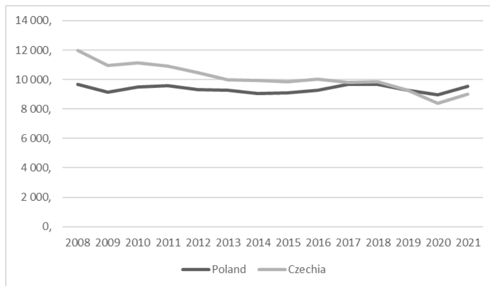
Figure 5. Greenhouse gases emissions from production activities (kg per capita) in Poland and the Czech Republic, 2008-2021
